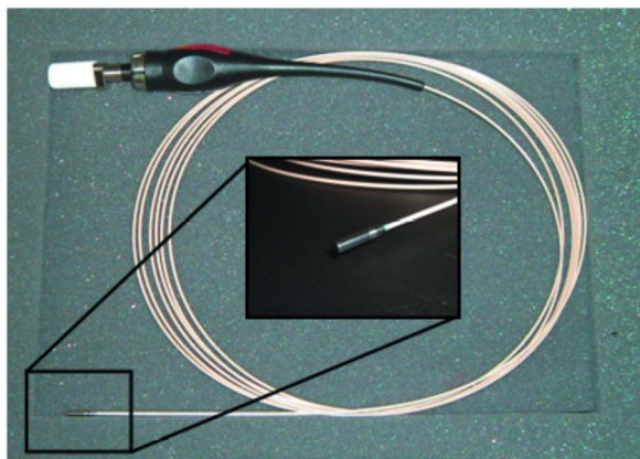
Fig. 1 Catheter-based reflectance-type laser-scanning confocal microscope (Mauna Kea Technologies, Paris, France; Fujinon, Saitama, Japan).
