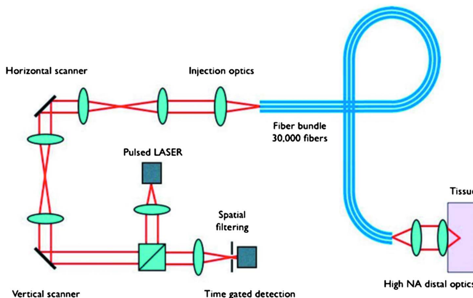
Fig. 2 Schema of the catheter-based reflectance-type laser-scanning confocal microscopy.
