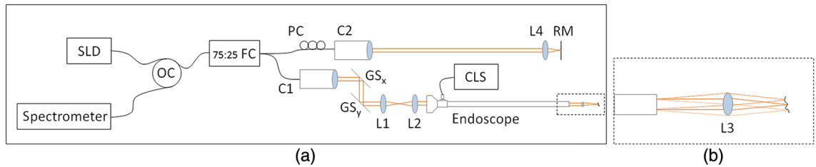
Fig. 3 (a) Scheme of the principle OCT setup. SLD, 5-mW superluminescent diode with \lambda_{center} = 835 nm and FWHM = 50 nm; OC, optical circulator; FC, wideband fiber coupler with a coupling ratio of 75:25; C1 and C2, collimators; GS, galvanometer scanners; L1–L4, lenses; endoscope, endoscope from Karl Storz GmbH and Co. KG; CLS, cold-light source; PC, polarization controller; RM, reference mirror; spectrometer, line rate of 11.88 kHz. (b) Telecentric imaging is realized by an additional lens L3 mounted on the distal end of the commercial endoscope at 4 mm distance by a custom adapter made of stainless steel.
