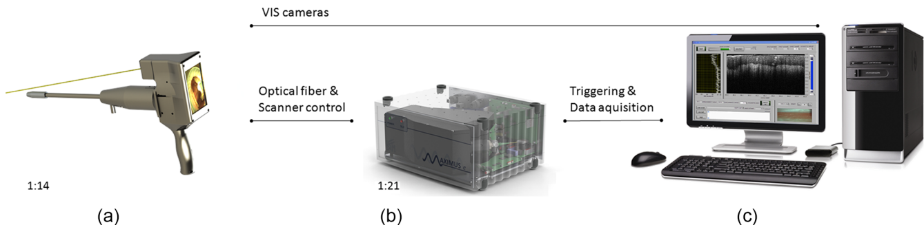
Fig. 4 Scheme of the measurement setup for the endoscopic investigation of the oral cavity equipped with (a) the EOCCT probe with integrated scanning sample arm, (b) the base OCT device with built-in SLD, spectrometer, partial fiber optics and system electronics, and (c) a personal computer for the control and triggering of the electronic components as well as the data display and acquisition.
