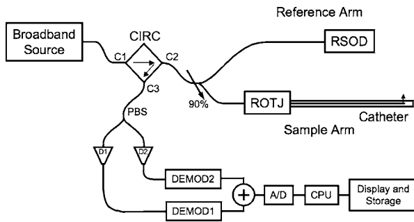
Fig. 1 Schematic of the time-domain intracoronary optical coherence tomography system. Polarized, broad-bandwidth light passes through a circulator (CIRC, port C1 to port C2) and is split into reference and sample arms via a 10/90 fiber optic beam splitter. The optical path length (group delay) of the reference arm is scanned by translating the galvanometer of the rapidly scanning optical delay (RSOD) line. Sample arm light is coupled into the catheter by a rotating optical junction (ROTJ). Light returned from the reference and sample arms is combined at the splitter and transmitted back to the circulator at port C2. The circulator then passes this light through port C3 to a polarizing beam splitter (PBS). The two orthogonal polarization states are detected separately by photodiodes D1 and D2. The two signals are demodulated and summed to create the final output signal, which is digitized (A/D) and transferred to the CPU. Detection of the fringe patterns created by sample and reference arm interference allows one radial scan (A-line) to be constructed that maps tissue reflectivity axial or depth location. A cross-sectional image is generated by repeating this process at successive transverse locations on the sample while the ROTJ rotates the internal components of the catheter.
