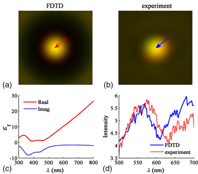
Fig. 5 Bright-field full-color reflection images of a 1- \mu\text{m} -diameter gold microsphere on a glass slide (a) synthesized by Angora and (b) experimentally obtained; (c) complex-valued permittivity profile of gold in the optical range assumed in the Angora model; (d) comparison of Angora-computed and experimentally measured wavelength-dependent spectra at the center pixels of the microsphere.
