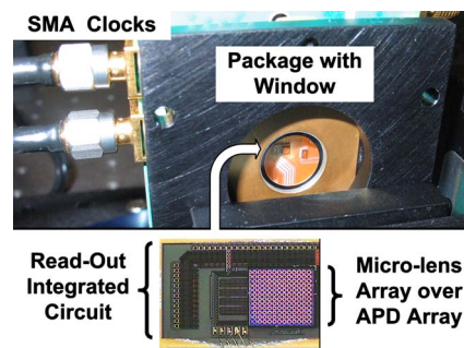
Fig. 4 Fully packaged photon-counting detector in test setup. Inset: Completed detector is about 3 \times 2 mm.
