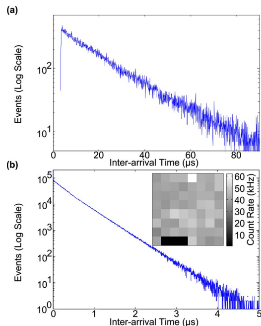
Fig. 2 Interarrival-time histograms of unilluminated APD firings for (a) a single detector and (b) 64 detectors. Inset: map of average dark count rate per detector.
