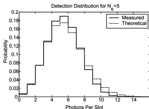
Fig. 3 Probability distribution of number of detected APD firing events per time slot with pulsed laser illumination at a fixed power level, showing multiphoton sensitivity.
