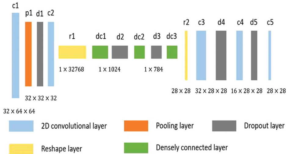
Fig. 2 The diagram of the proposed HNN model.
