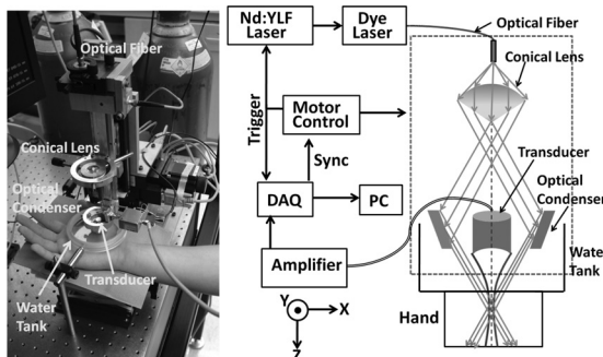
Fig. 1 Photograph and schematic of the photoacoustic microscope. (Color figures available online only.)
