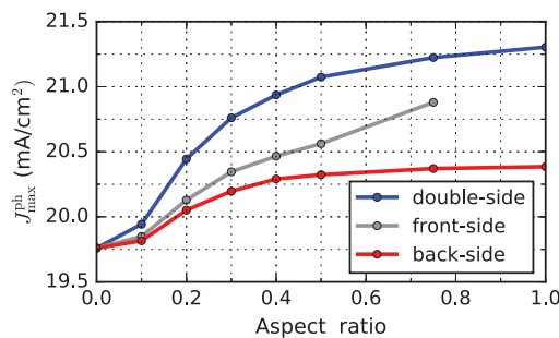
Fig. 6 The maximum achievable matched current density J_{\text{ph}}^{\text{max}} after thickness optimization shown in dependence of the aspect ratio for the three architectures shown in 3. The corresponding optimal effective perovskite layer thicknesses are shown in Table 2.
