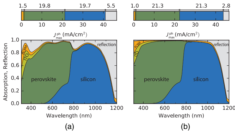
Fig. 7 Absorption profile and associated theoretical current density for the (a) planar and (b) fully textured architecture with a = 1.0 . With a maximum achievable current density of 21.3 \text{mA/cm}^2 for each absorber cell, we have a power conversion efficiency of 31.8%.
