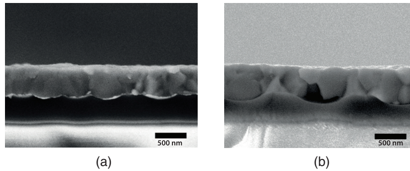
Fig. 1 5 kV SEM micrograph images of perovskite on sinusoidal substrates with (a) P = 500 nm and a = 0.16 , (b) P = 750 nm and a = 0.27 . The bright layer between substrate and perovskite represents the evaporated silver.
