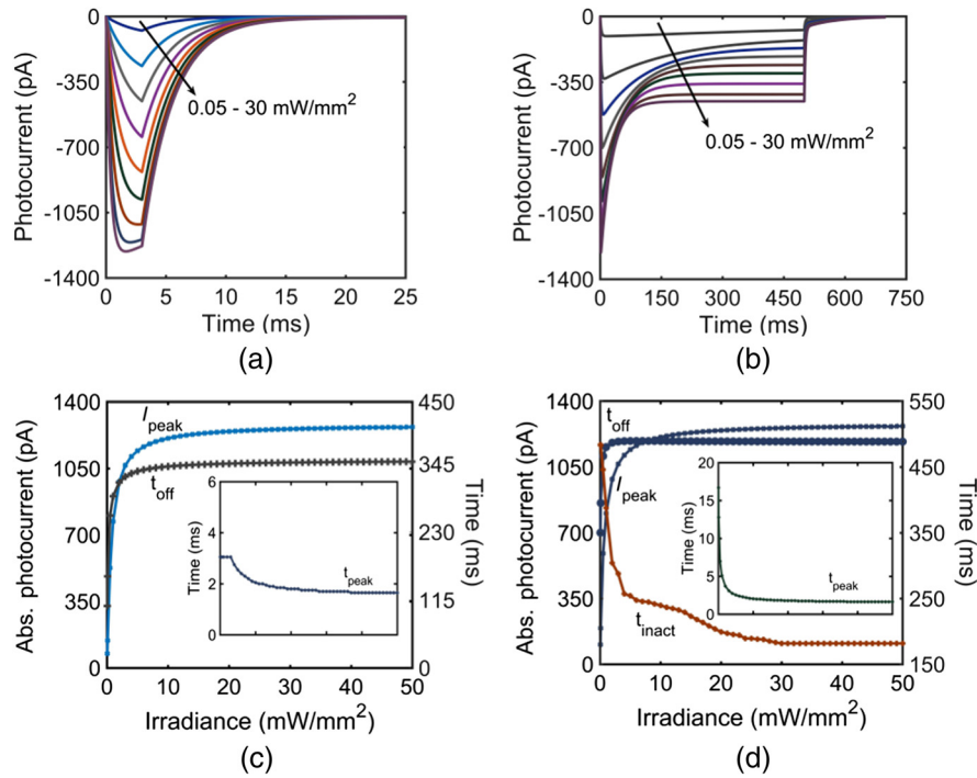
Fig. 3 Effect of irradiance on the photocurrent of vf-Chrimson. (a) At irradiances 0.05, 0.2, 0.4, 0.7, 1.2, 2, 4, 10, and 30 \text{mW}/\text{mm}^2 , at \lambda = 594 \text{ nm} , and 3-ms pulse width; (b) corresponding variation at 500-ms pulse width. (c) Variation in I_{\text{peak}} and t_{\text{off}} with irradiance under 3-ms pulse stimuli. Inset: corresponding t_{\text{peak}} variation with irradiance (on the same scale). (d) Variation of I_{\text{peak}} , t_{\text{off}} , and t_{\text{inact}} with irradiance at 500-ms pulse stimuli. Inset: corresponding variation of t_{\text{peak}} with irradiance (on the same scale).
