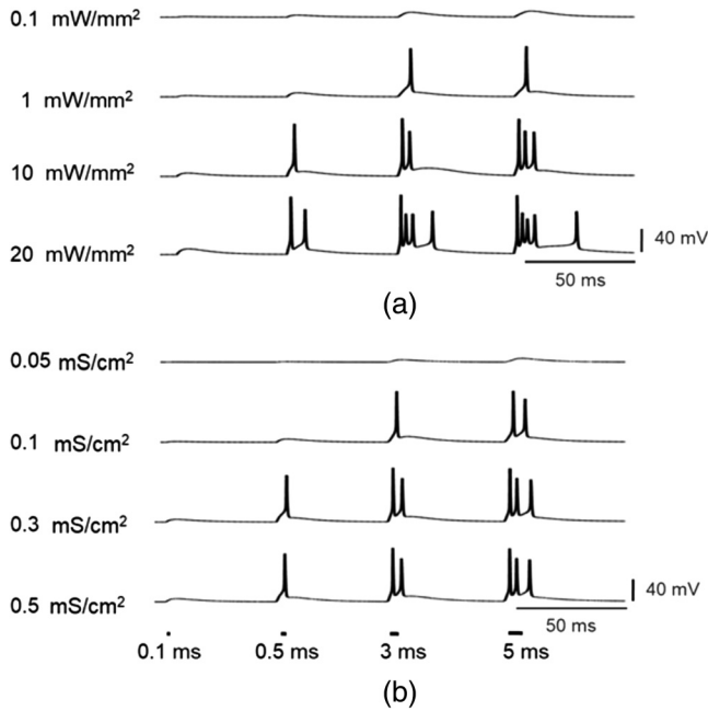
Fig. 13 Effect of irradiance, pulse width, and expression level on the spiking fidelity in vf-Chrimson-expressing interneurons. At \lambda = 565 nm and (a) irradiances when g_0 = 0.25 mS/cm 2 and (b) expression level at I = 10 mW/mm 2 .
