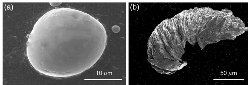
Fig. 1 Morphology of representative surrogate Ti particles from (a) commercially available Ti spheres and (b) homemade Ti filings. The Ti sphere shown has a diameter of 22 \mu\text{m} . The length of the Ti filings shown is \sim 150 \mu\text{m} ; its width ranges between 45 and 55 \mu\text{m} .
