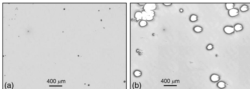
Fig. 2 Optical images of the \text{Al}_2\text{O}_3 capping layer surface: (a) with spherical Ti particle sprinkled on before laser shot and (b) after a single laser shot.
