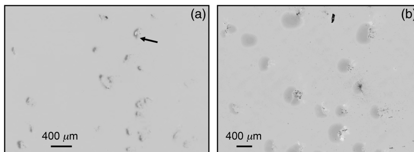
Fig. 4 Optical images of the capping layer surface after one laser shot at the presence of irregularly shaped Ti filings: (a) Al 2 O 3 surface and (b) SiO 2 surface.
