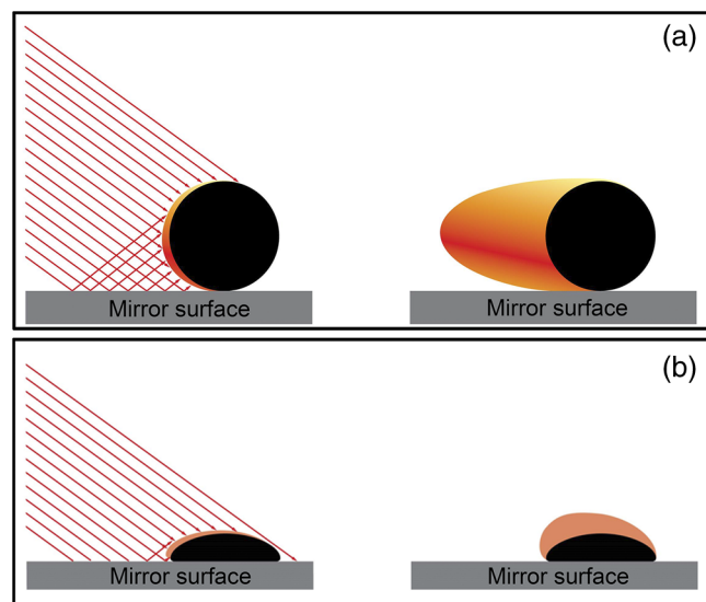
Fig. 6 Schematics showing the laser-induced plasma formation and particle recoil on reflective surface with (a) a spherical Ti particle and (b) an oblate-shaped Ti particle.
