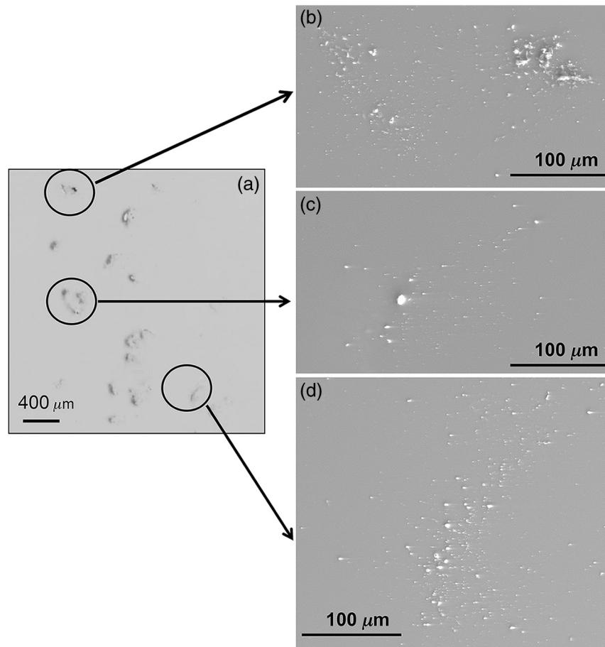
Fig. 5 Microscope images of particles on the \text{Al}_2\text{O}_3 capping surface after one laser shot at the presence of irregularly shaped Ti fillings: (a) optical image showing the surface features and (b)–(d) SEM images showing a closer view of the specific sites marked in (a). The sites are clearly from fragmented Ti particles and are not surface damage.
