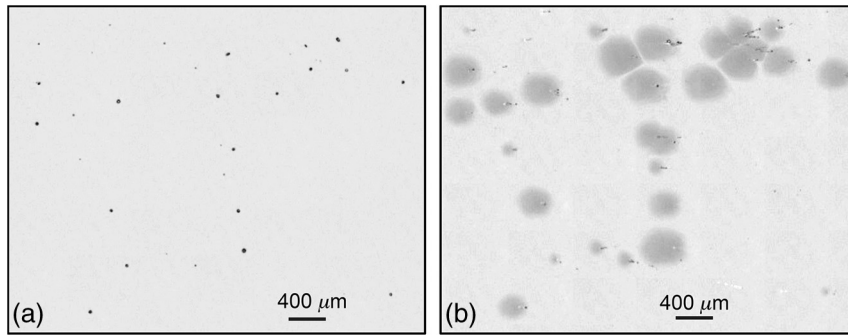
Fig. 3 Optical images of the SiO 2 capping layer surface: (a) with spherical Ti particle sprinkled on before laser shot and (b) after a single laser shot.
