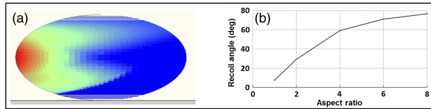
Fig. 7 (a) Absorbed intensity on the surface of an ellipsoidal particle (aspect ratio 2:1) and (b) recoil angle versus aspect ratio.
