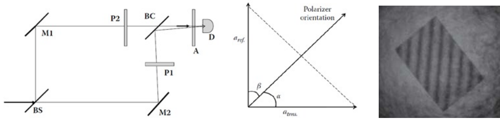
Figure 3.6.1 Left Diagram: Two orthogonally polarized beams were generated in the two arms of a Mach-Zehnder interferometer (MZI) and were superposed non-collinearly on the beam-combiner (BC). (The MZI is in fringe mode when only a detector array can register spatial fringe intensity variation.) However, with orthogonally polarized beams, it does not produce any fringes until a polarizer is inserted bisecting the two orthogonal direction of polarizations. Right Diagram: The recorded fringes visible only within the boundary of the Polaroid. No fringes were visible outside boundary of the Polaroid (see Fig.1.3 in ref.9).
