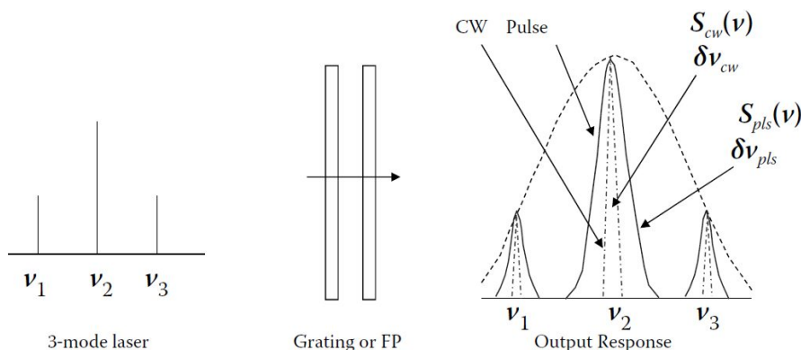
Figure 3.2. The output response of a spectrometer shows fringes of finite width (dashed vertical curves on the right diagram) even when the input signal is infinitely narrow three CW laser modes (shown on the left). We correctly recognize this width as the CW instrumental response function. The output response would be wider (solid vertical curves) if we allow a simple screen to chop out a single pulse from the 3-mode CW laser. We should recognize this widening as the pulse response function of the spectrometer, rather assuming that the width is due to existence of Fourier frequencies in the chopped pulse [see Fig. 1.1 in ref.9].
