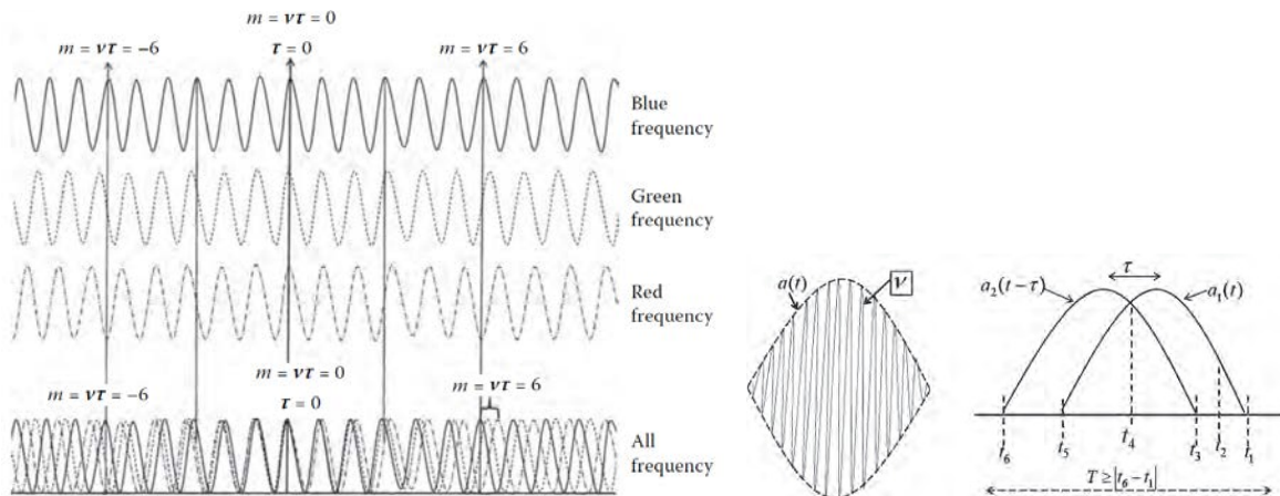
Figure 3.3. Left Diagram (see Fig.1.2 in ref.9): Some of the most precise measurements using optical interferometry is done by using broadband or white light. Highly “incoherent” white light can produce quantifiable fringes for measurements for small path differences (see the very bottom sketch above). The fringes wash out for increasing relative path differences. This can be appreciated from the bottom of the left figure. The red, green, and blue fringes have different spatial frequencies. When they all are present simultaneously, the fringes show increasing wash-out effect as one move further from the “zero-path-delay” position. Right Diagram [see Fig.6.1 and 6.2 in ref.9]: In pulse autocorrelation experiments, a single pulse is replicated and superposed with different relative delays. Replicated pulses are phase steady; not incoherent. Fringe visibility degrades because unequal amplitudes are superpose, not due to physical presence of Fourier frequencies.
