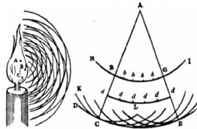
Figure 3.1.1 Diagrams sketched by Christian Huygens in his book [10] explaining the intrinsic properties required by waves to keep on propagating perpetually energized by cosmic ether as a tension field. Each point on every wave front functions as a source for a secondary wavelet. He also explicitly stated that his secondary wavelets keep on expanding through each other without influencing (interacting with) each other. This is Non-Interaction of Waves (NIW).
