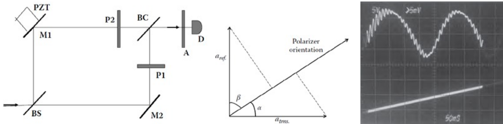
Figure 3.6.2 An MZI in collinear superposition mode for a pair of phase-steady orthogonally polarized light beams. The detector can observe the superposition effect only when one of the mirrors is scanned to introduce relative phase delay between the two beams along with a polarizer before the detector. The two superposed beams on the detector are now parallel, dictated by the polarizer. The detectors now can respond to the superposition effect. The beam combiner (BC) remains passive to the orthogonally polarized beams as in the case for non-collinear superposition above (Fig.3.6.1).
