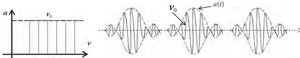
Figure 3.4. Mode lock theory in basic textbooks sums the amplitudes of a periodic array of phase-steady frequencies (left diagram) to obtain a continuous train “mode locked” pulses. Clear implication is that wave amplitudes are interacting and re-grouping their energies, which violates the NIW property of light, as explained earlier. In reality, it is the time-periodic intensity response function of the intra-cavity mode-locking device, which functions as a time gating device, enforcing the intra-cavity gain of a train of reverberating light pulses. [see Fig.7.1 in ref.9]
