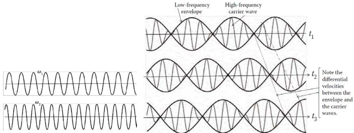
Figure 3.5. Left Diagram: Two phase steady continuous waves. Right Diagram: Mathematical summation of two phase-steady continuous cosine waves for two different carrier frequencies will give a mathematical wave with a new carrier frequency of value equaling the mean of the sum frequencies modulated by an envelope wave, which is the mean of the difference frequency. Since materials impose frequency dependent velocities, one mathematically finds that the envelope wave travels with a group velocity that is different from the phase velocity of the resultant carrier wave. This is the standard textbook theory. However, it violates the NIW property of waves, underscored earlier. The two component waves will co-propagate unperturbed by each other, as long as the medium supporting the waves remain linear and non-interacting with the waves [see Fig.8.4 in ref.9].
