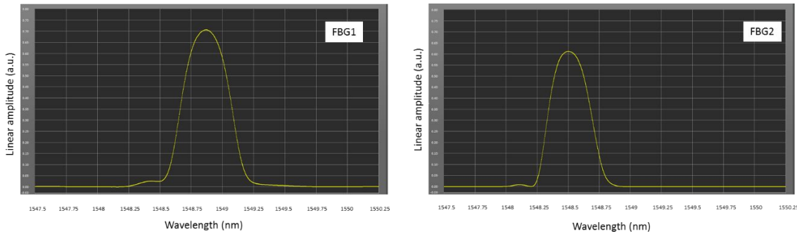
Fig. 7. Spectral response of two fs-FBG samples connected to two FAZ I4 interrogator channels
