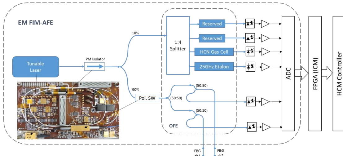
Fig. 1. Schematic diagram of the HSB Fiber Optic Interrogator Section
