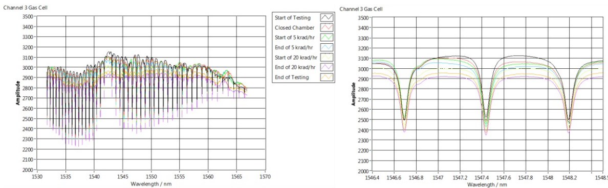
Fig. 5. Overall Spectral Response of the Gas Cell Lines in the C-band (left), Zoomed in for absorption lines P Branch 06, P Branch 07, and P Branch 08 (right)
