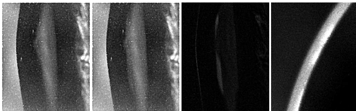
Fig 5: IR long exposure image of the optical fiber: laser off, laser on, and the difference between the two. The last image is the reference for the quantification of the flux taken in the same conditions in our laboratory.
