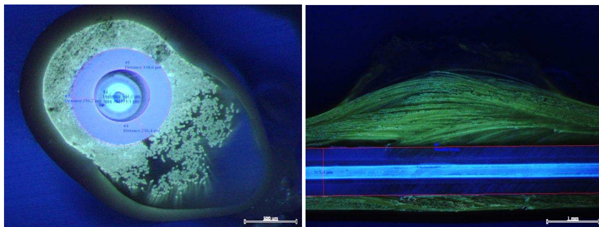
Fig 7: Cross-section under UV light to identify the 5 protection layers and the depth of damage
