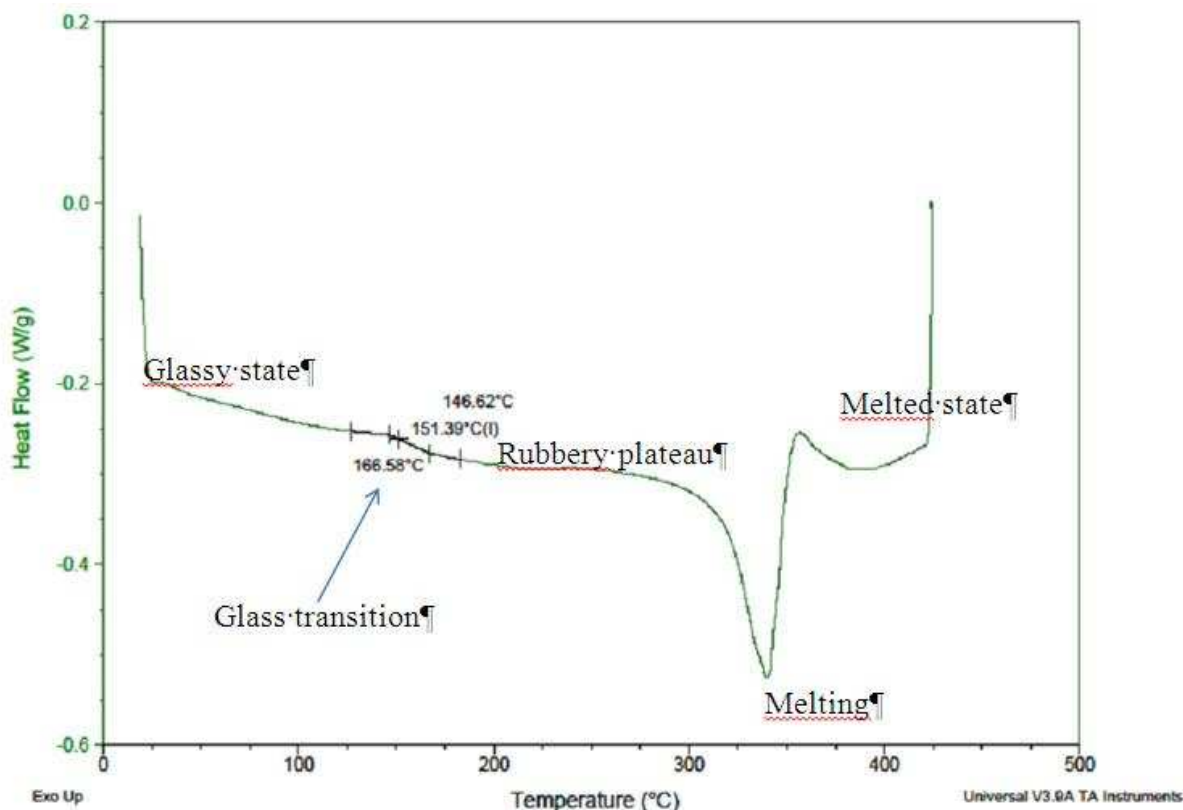
Fig 8: Differential Scanning Calorimetry measurement on the sheath
