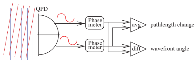
Fig. 6. Differential wavefront sensing principle.
