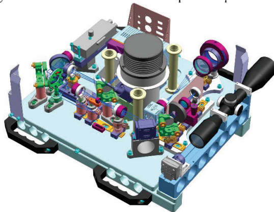
Figure 2: Optomechanical STB design (excluding the PAA stage)
